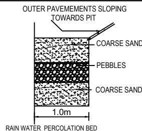
RAIN WATER PERCOLATION BED
