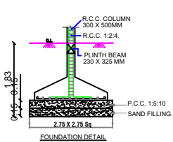
FOUNDATION DETAIL
