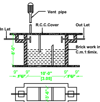
SEPTIC TANK DETAILS (NOT TO SCALE)
