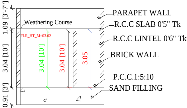
SECTION ON"AB"
