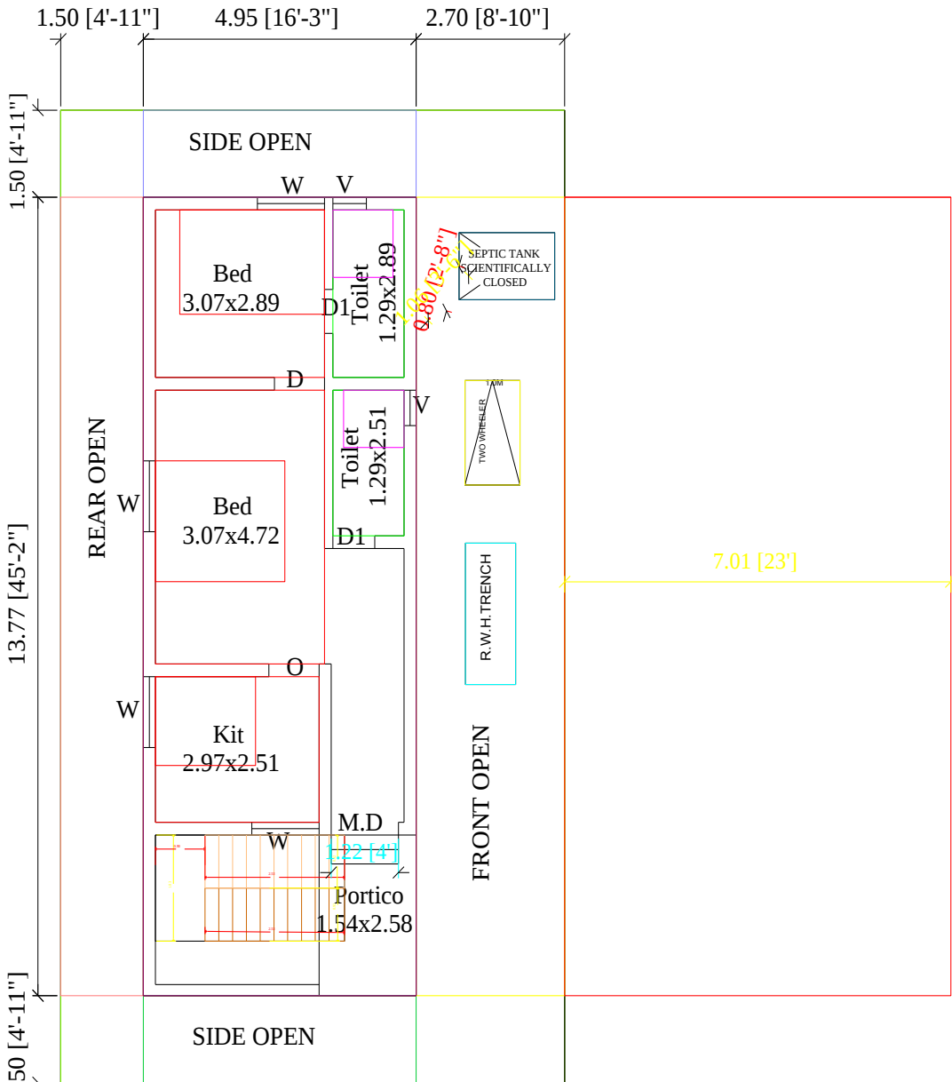
PRO.GROUND FLOOR
