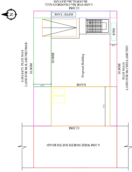
SITE PLAN (SCALE - 1:100)
