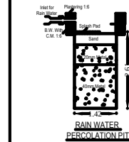
RAIN WATER PERCOLATION PIT
