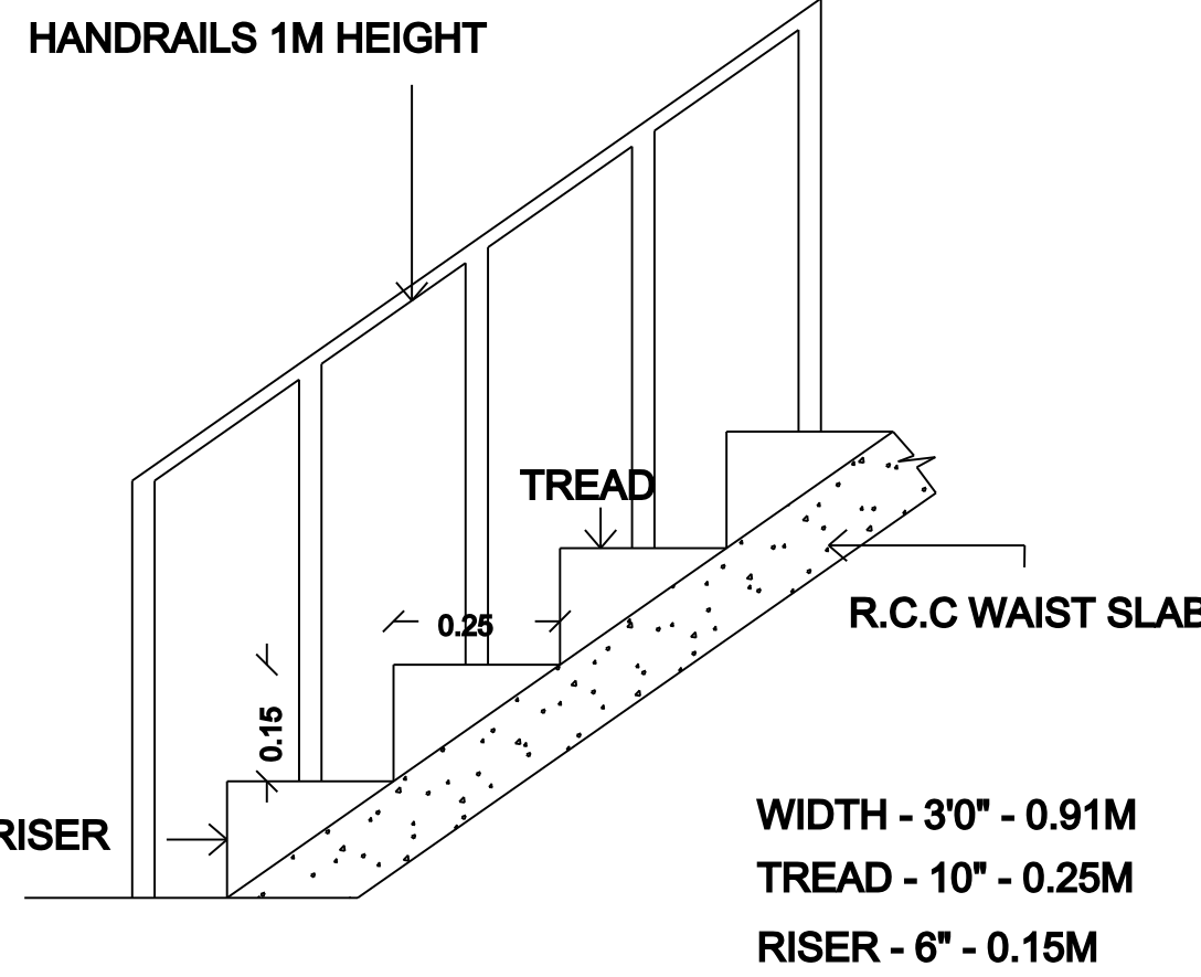
STAIRCASE DETAILS
