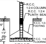
FOUNDATION DETAIL
