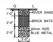
RAIN WATER PERCOLATION PIT (NTS)
