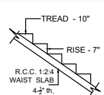
STAIRCASE DETAILS (NTS)
