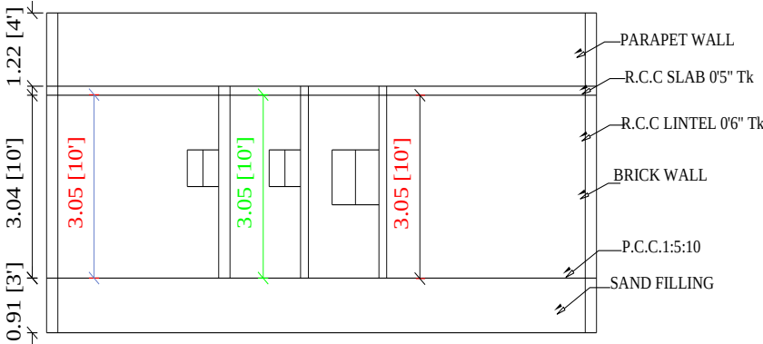
SECTION ON"AB"
