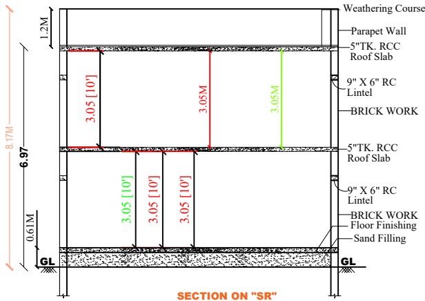
SECTION ON "SR"
