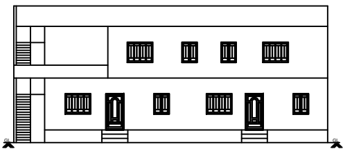
FRONT ELEVATION (SOUTH FACING)
