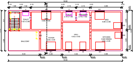
PRO.FIRST FLOOR PLAN
