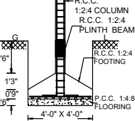
FOUNDATION DETAIL
