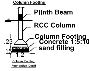
Column Footing Foundation Detail
