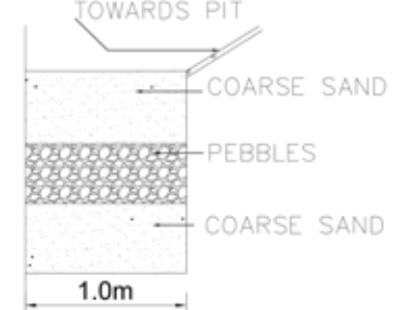
OUTER PAVEMENTS SLOPING TOWARDS PIT
