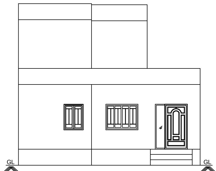
FRONT ELEVATION (EAST FACING)
