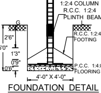
FOUNDATION DETAIL
