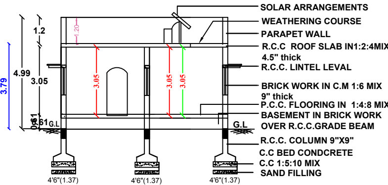
SECTION " AB "
