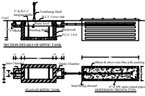
DETAILS OF SEPTIC TANK & DISPERSION TRENCH
