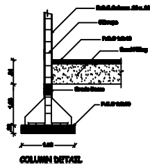
COLUMN DETAIL
