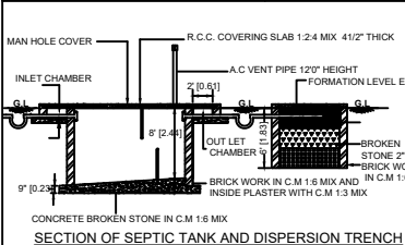
SECTION OF SEPTIC TANK AND DISPERSION TRENCH
