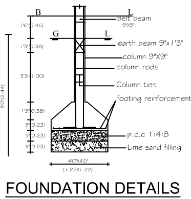
FOUNDATION DETAILS
