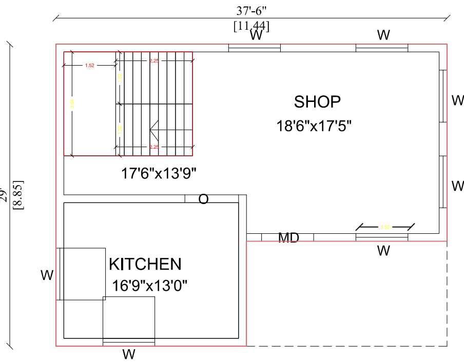
EXG., GROUND FLOOR PLAN
