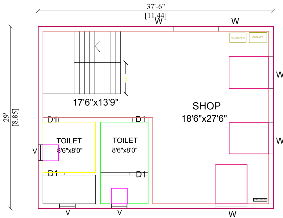
PRO., FIRST FLOOR PLAN
