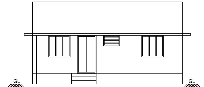
FRONT ELEVATION
