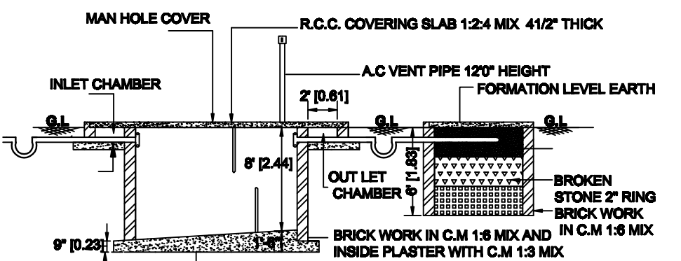
SECTION OF SEPTIC TANK AND DISPERSION TRENCH
