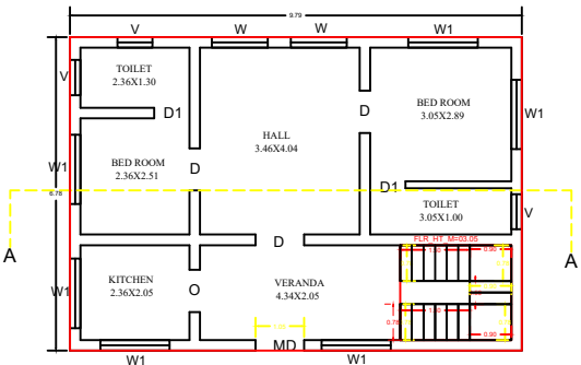
EXISTING GROUND FLOOR
