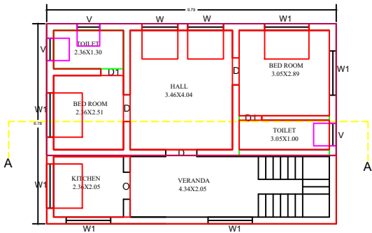
EXISTING & PROPOSED FIRST FLOOR
