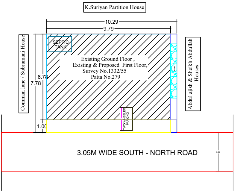
SITE PLAN
