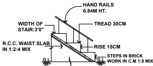
STAIR CASE DETAILS. (NOT TO SCALE)
