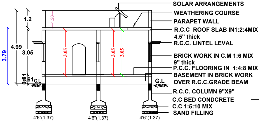
SECTION " AB "
