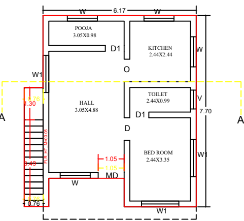
EXISTING GROUND FLOOR (WEST FACING)
