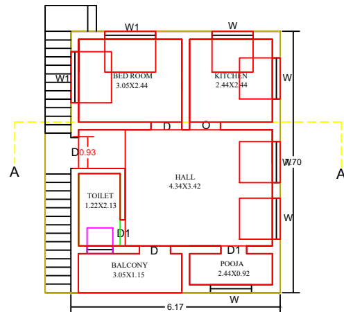
PROPOSED FIRST FLOOR (WEST FACING)
