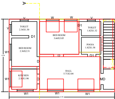
EXISTING & PROPOSED FIRST FLOOR
