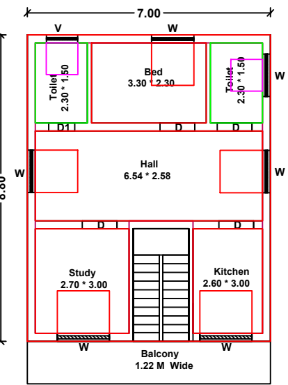
Additional Proposed II nd Floor
