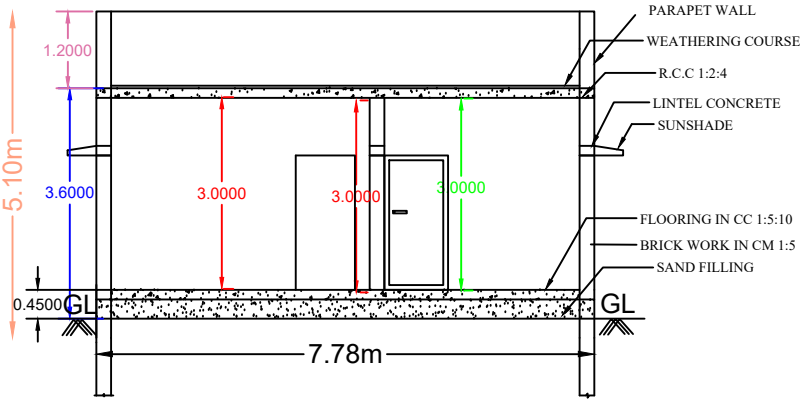
SECTION AB
