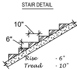
STAIR DETAIL
