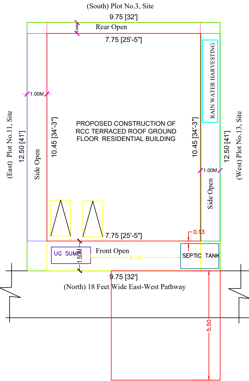
SITE PLAN
