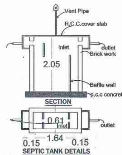
SECTION SEPTIC TANK DETAILS
