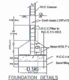
FOUNDATION DETAILS
