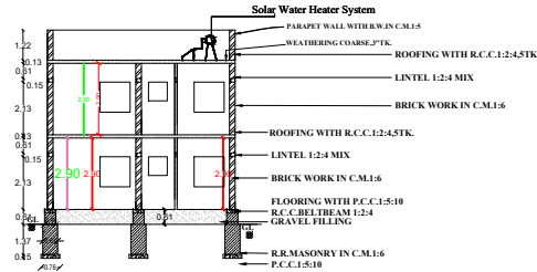
SECTION FACING ON A&A
