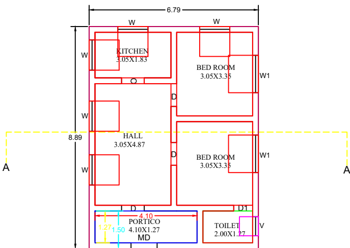
GROUND FLOOR
