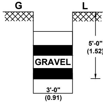
TRIAL PIT (NTS)
