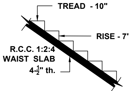
STAIRCASE DETAILS (NTS)
