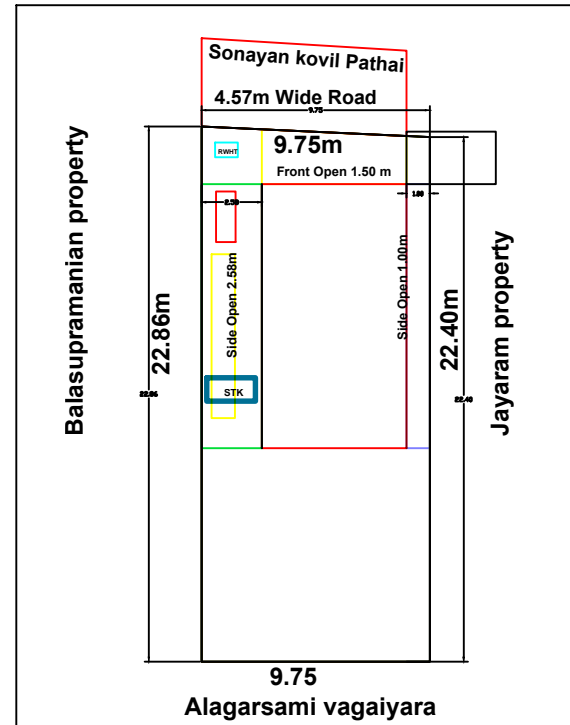
SITE PLAN
