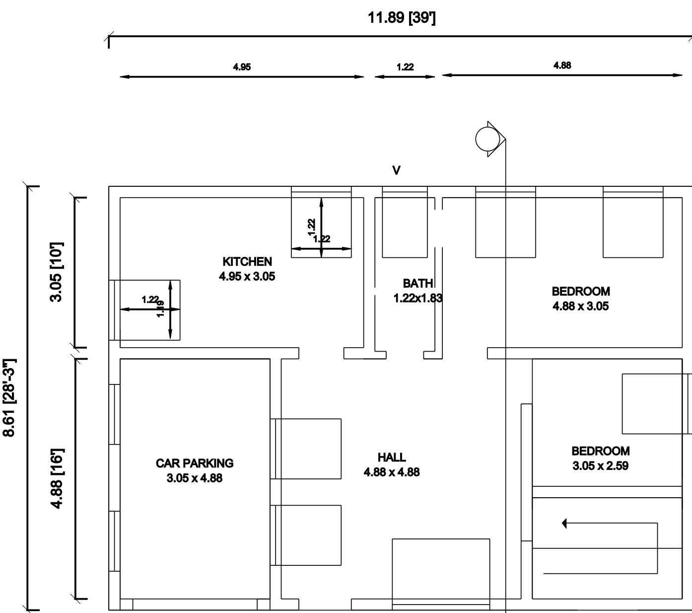
PRO.GOUND FLOOR PLAN
