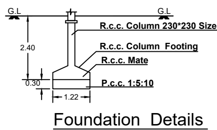
Foundation Details
