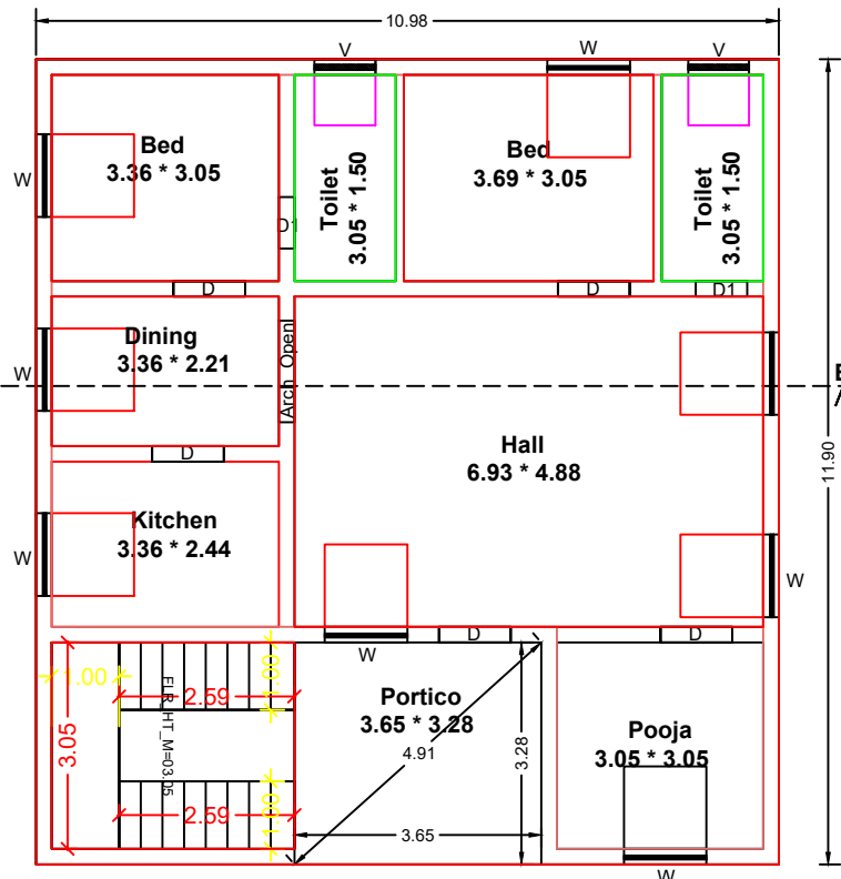
Proposed Ground Floor East Facing
