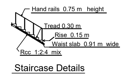
Staircase Details
