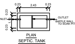
PLAN SEPTIC TANK
