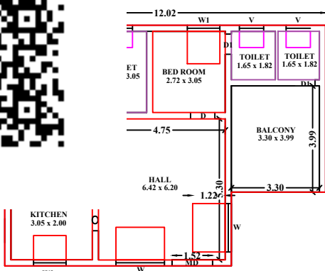
PRO.FIRST FLOOR PLAN
