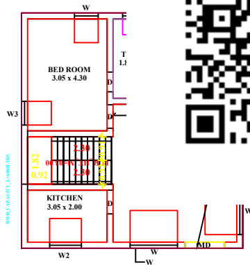
PRO.GROUND FLOOR PLAN
