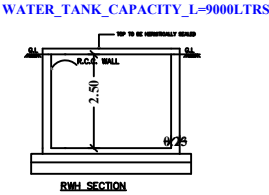
RWH SECTION
