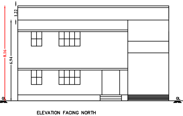
ELEVATION FACING NORTH
