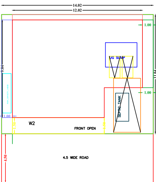
SITE PLAN
