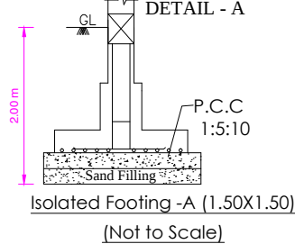
FOUNDATION DETAIL - A
