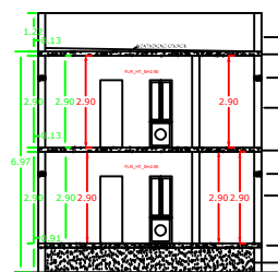
SECTION ON K-S
