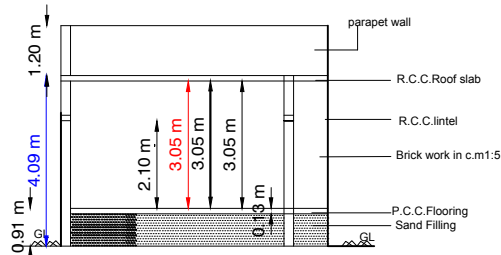
SECTION-"SR"
