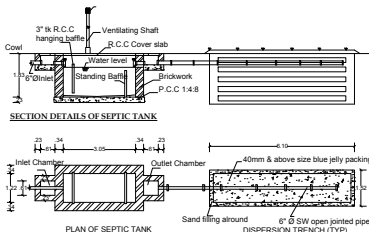
DETAILS OF SEPTIC TANK & DISPERSION TRENCH
