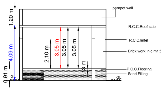
SECTION-"SR"
