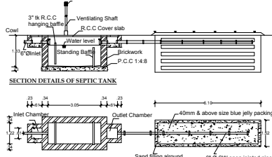
DETAILS OF SEPTIC TANK & DISPERSION TRENCH
