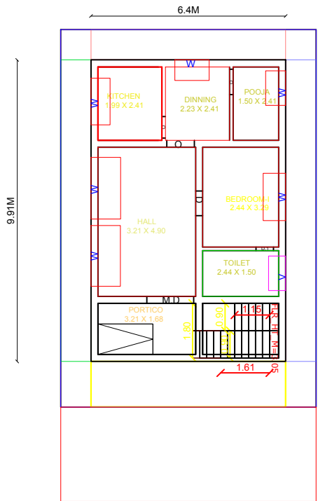
JND FLOOR
