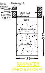
RAIN WATER PERCOLATION PIT
