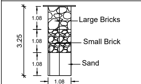
SECTION OF RAIN WATER COLLECTION PITS (NTS)
