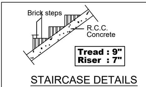
STAIRCASE DETAILS
