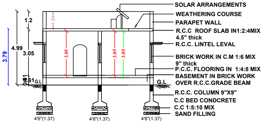
SECTION " AB "
