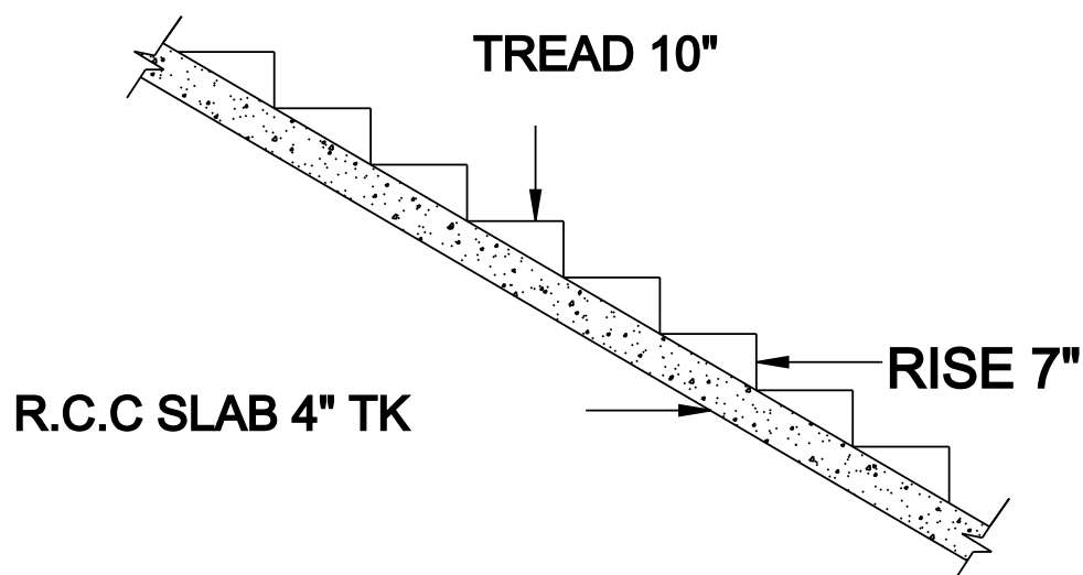
STAIRCASE DETAILS
