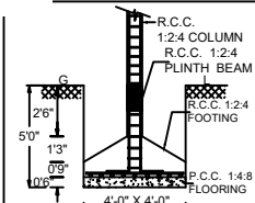
FOUNDATION DETAIL
