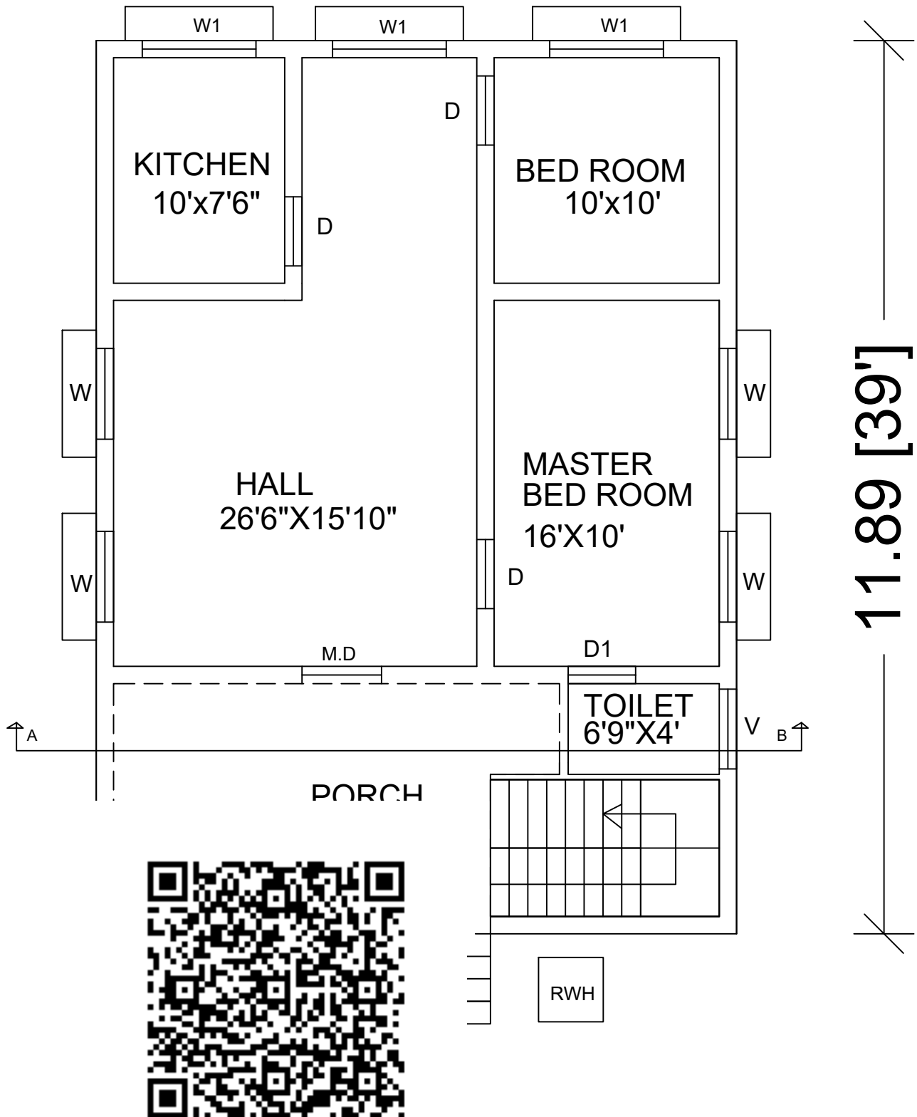
FRO. GROUND FLOOR PLAN
