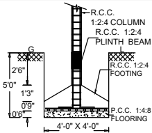
FOUNDATION DETAIL
