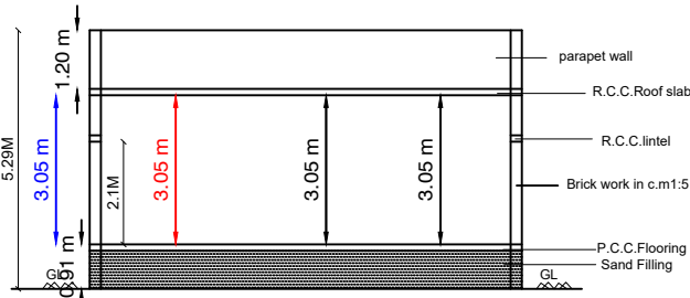
SECTION-"SR"
