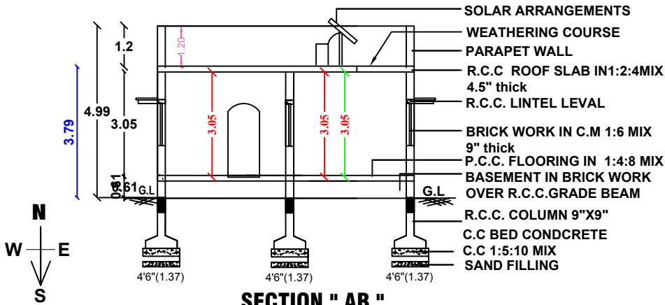
SECTION " AB "
