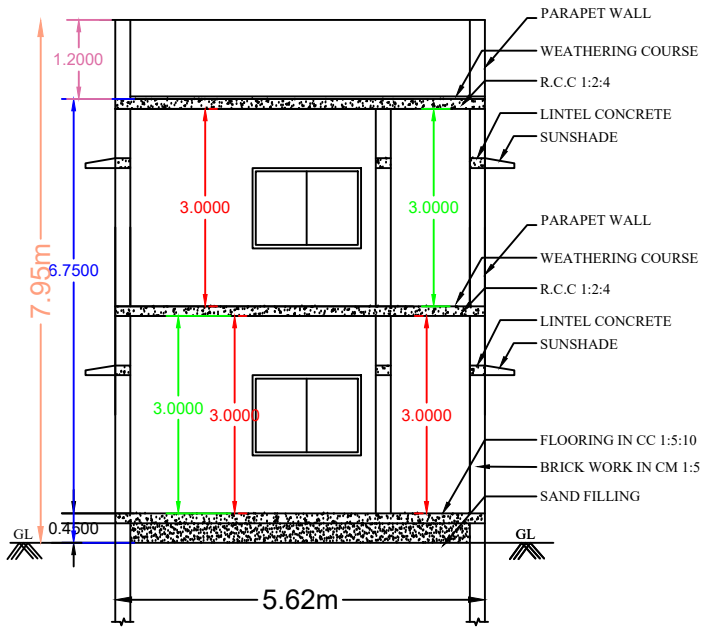
SECTION AB
