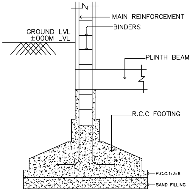
TYPICAL SECTION OF R.C.C COLUMN FOUNDATION
