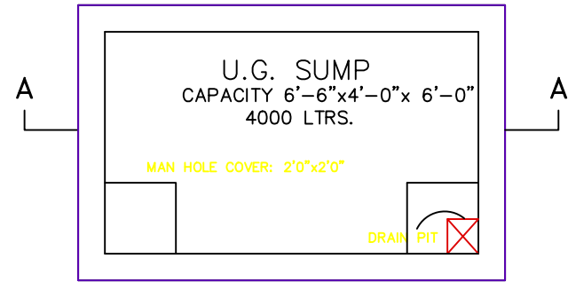
SUMP DETAIL
