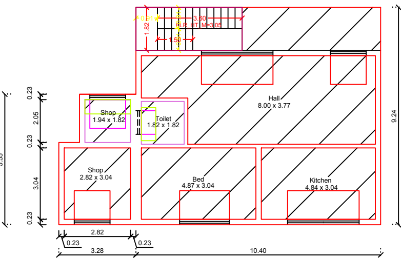
EXG.GROUND FLOOR PLAN
