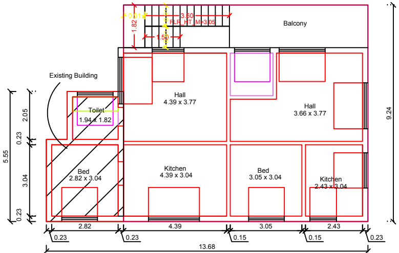
PRO. ADDITIONAL FIRST FLOOR PLAN
