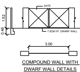
COMPOUND WALL WITH DWARF WALL DETAILS
