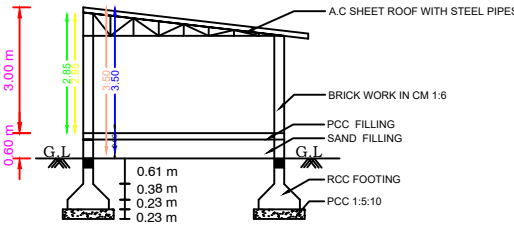
SECTION ON KA
